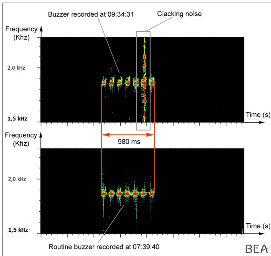
Figure 15 - buzzer spectral analysis
